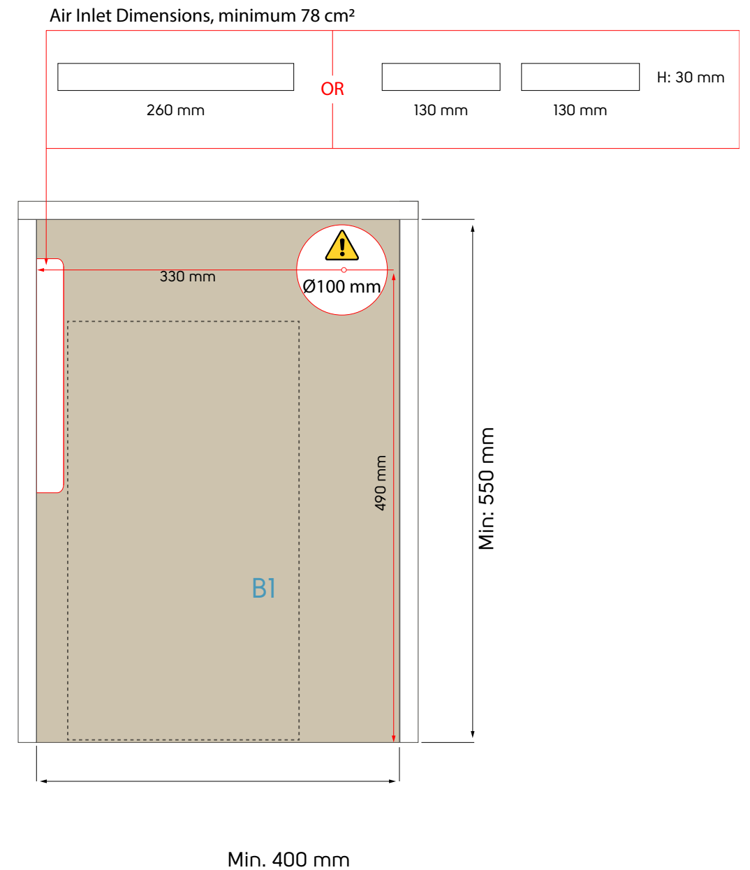
Top View
